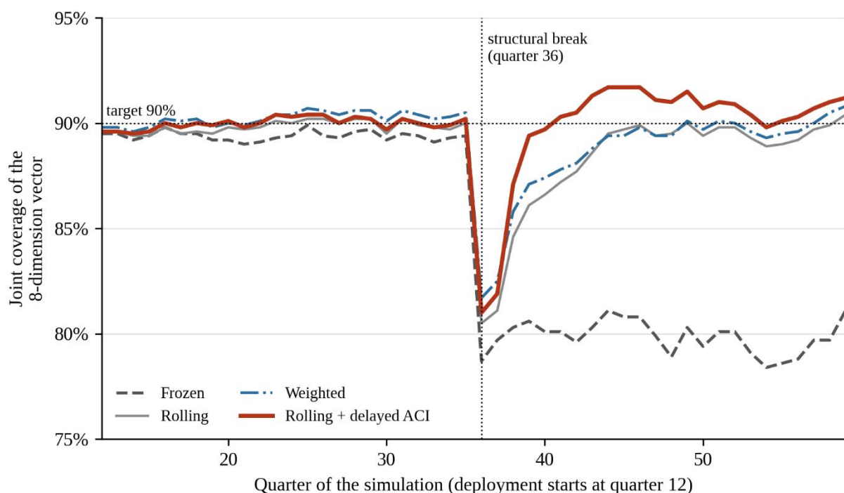
Figure 1. Joint coverage of the eight-dimension vector by quarter, mean of 200 replications. After the structural break at quarter 36, frozen calibration stays about 10 points under the 90% target, while delayed-feedback adaptation recovers in about four quarters. Simulation, seeds 1000 to 1199; deployment quarters 12 to 59.
