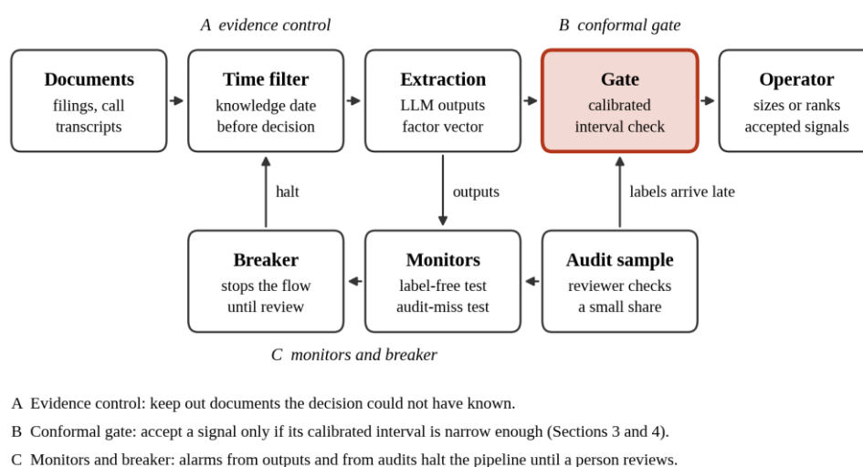
Figure 7. Deployment framework with three components around the extraction step: (A) evidence control, (B) the conformal gate, and (C) monitors and a circuit breaker. Only component B is evaluated in this paper.
