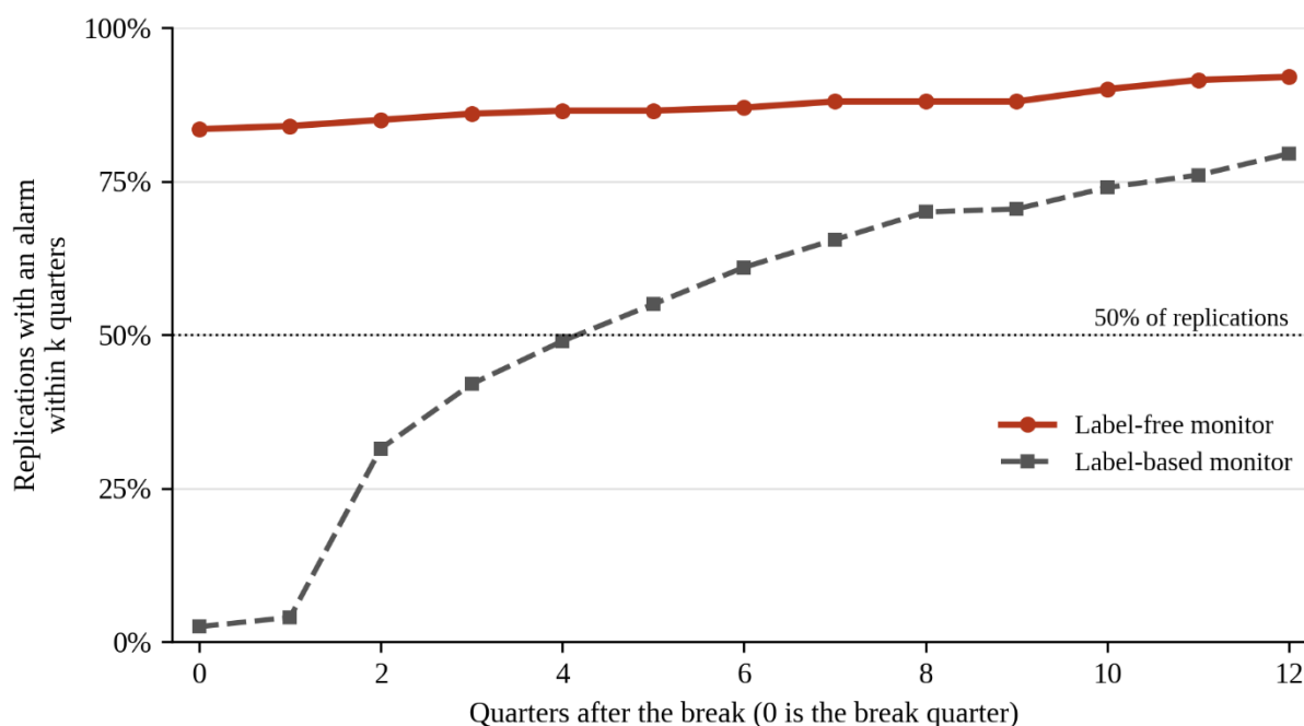
Figure 3. Share of replications with an alarm within k quarters of the structural break. The label-free monitor flags 83.5% of breaks in the quarter they occur, while label-based coverage monitoring needs about four quarters to reach 50%. Simulation, 200 replications; alarms counted from the break quarter (quarter 36).
