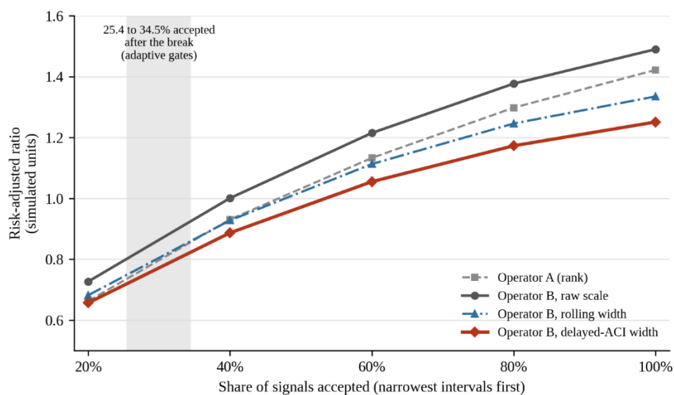
Figure 2. Risk-adjusted ratio against the share of signals accepted, for a rank operator and three width-scaled operators. The ratio rises with acceptance for every operator, and sizing by conformally calibrated width does worse than sizing by
