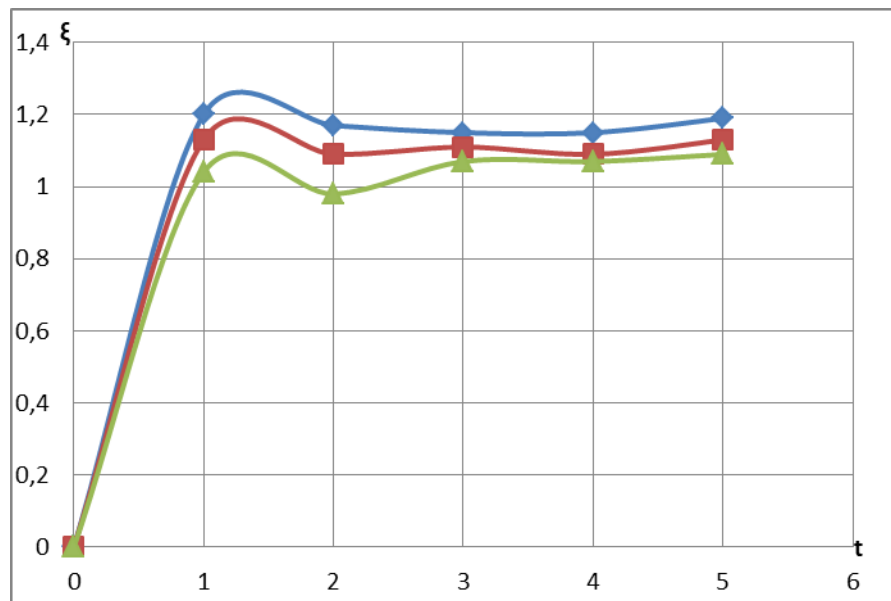
Figure 6. Graph of change of hydraulic resistance coefficient in plates over time.
