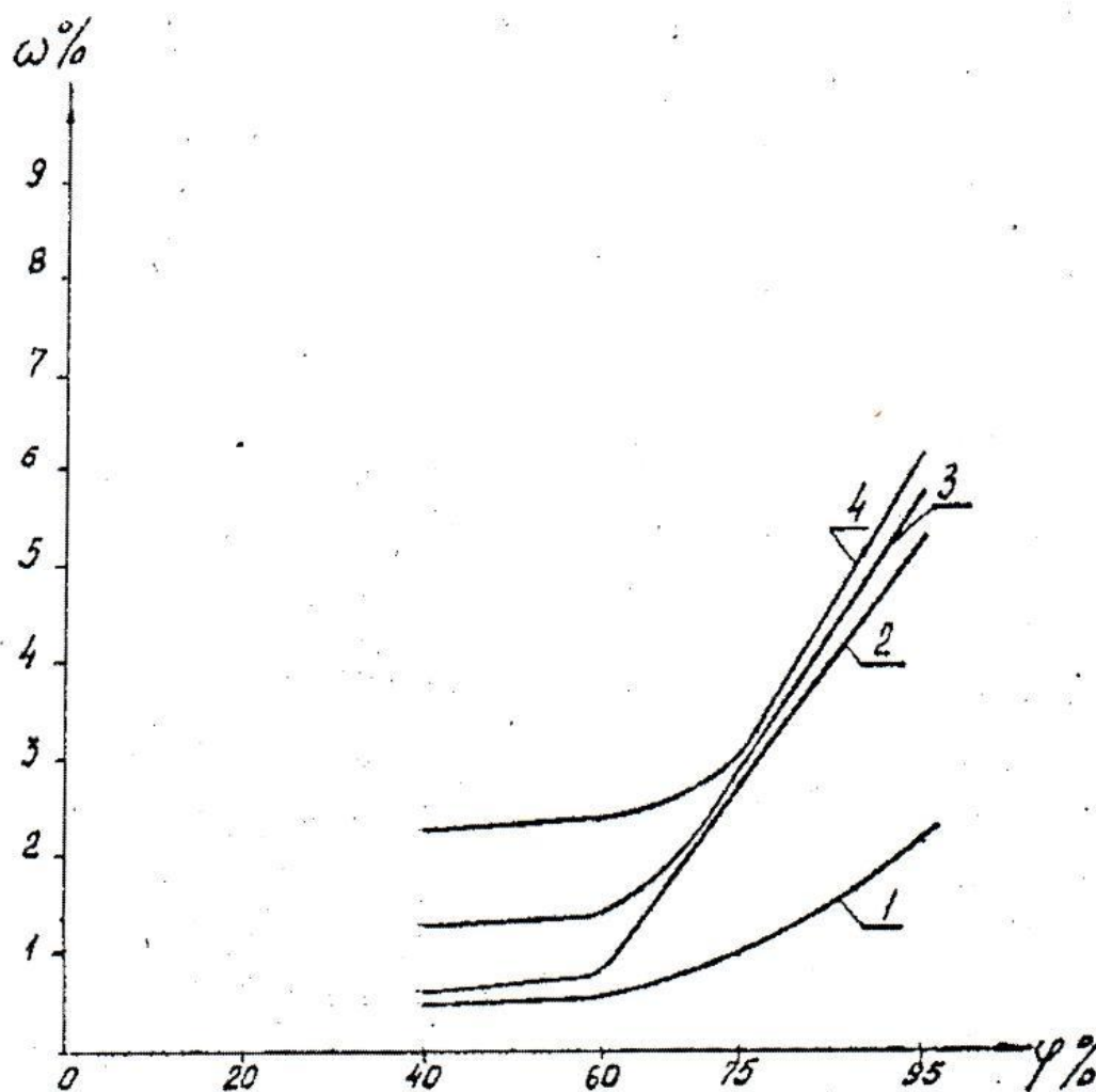
Rice. 1. Dependence of the sorption moisture content of building materials on the degree of salinity with sodium chloride.
