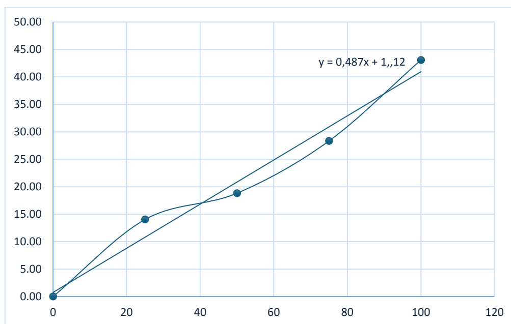
Figure 5. Relationship graph between ARF% and volume determined at 30 minutes of aqueous extracted Inula grandis .
