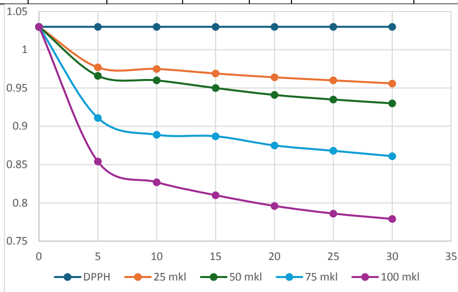
Figure 2. Graphical representation of the measured light absorption of blank and tested alcohol-extracted Inula grandis solutions spiked with DPPH solution ( Inula grandis alcoholic 10x).
