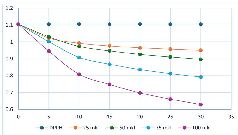
Figure 4. Graphical representation of the measured light absorption of blank and tested aqueous extracted Inula grandis solutions spiked with DPPH solution ( Inula grandis watery 10x).
