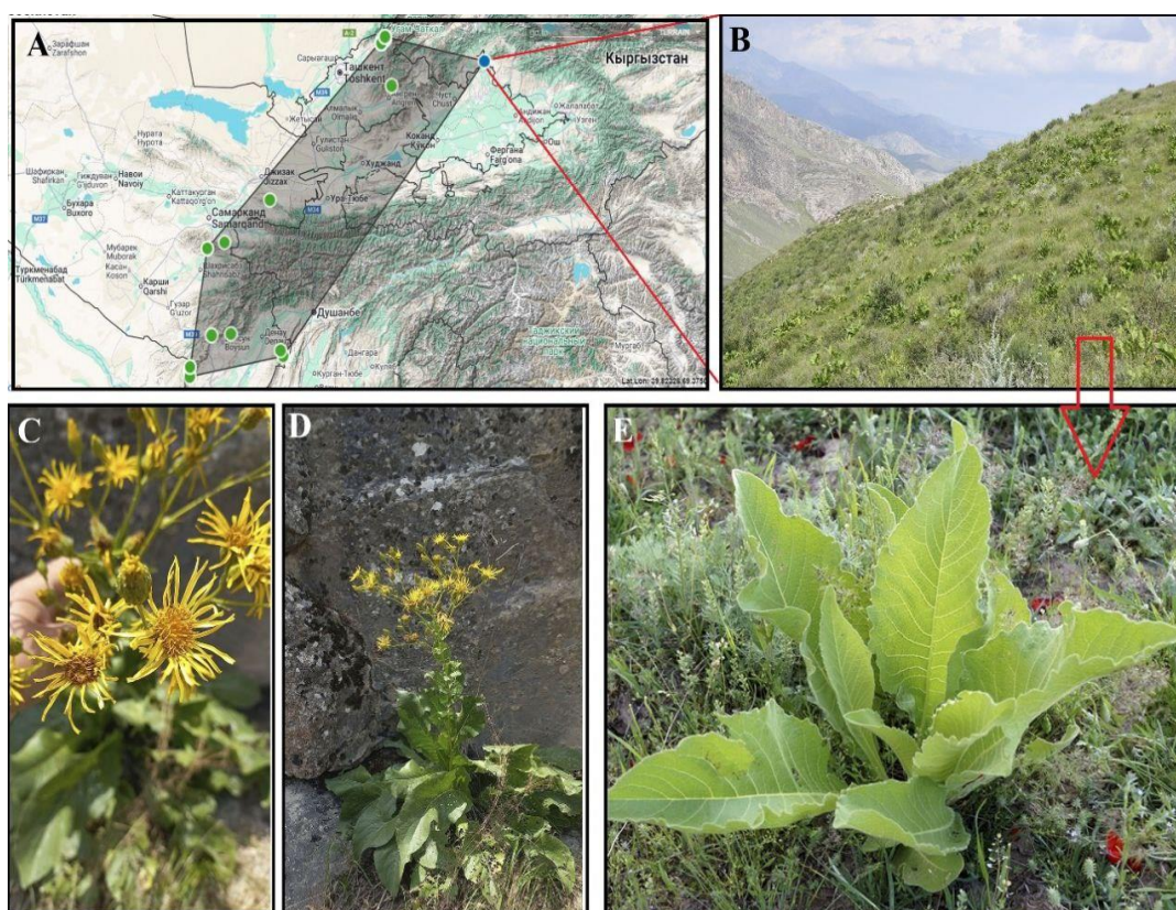
Figure 1. A) Distribution map of Inula grandis ; B) Ecology; C-D-E) Images of the plant in nature.
